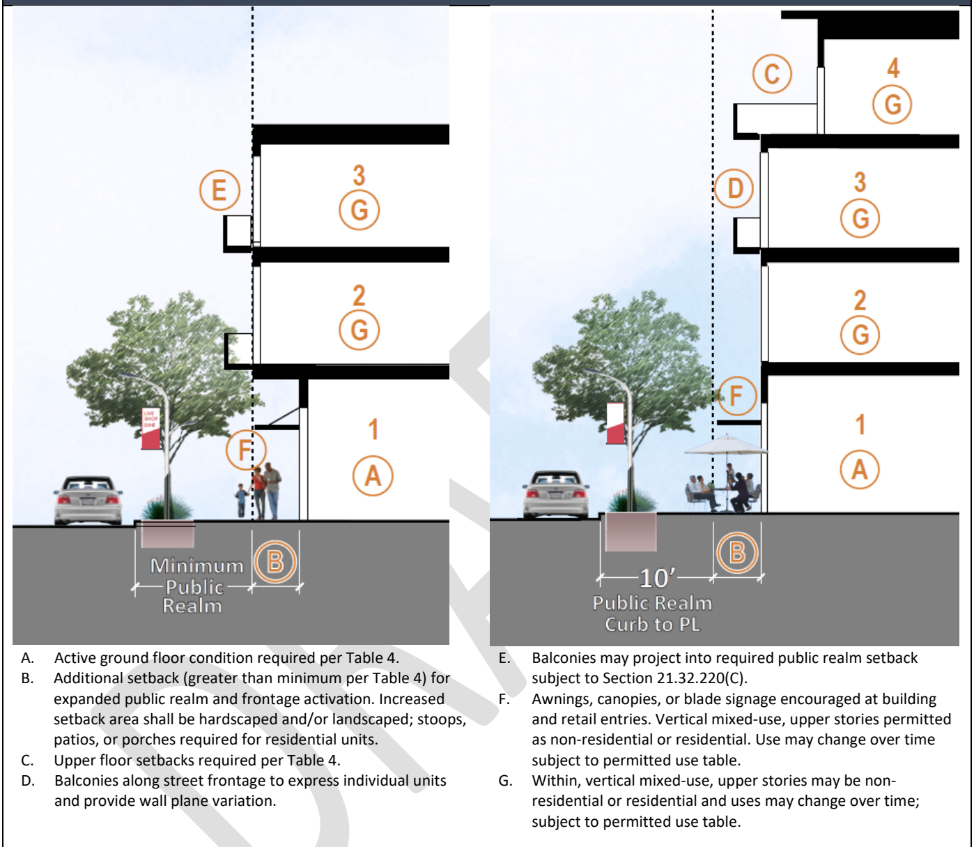
Figure 4 Building Placement & Activation Diagram – Three & Four Story Mixed-Use
