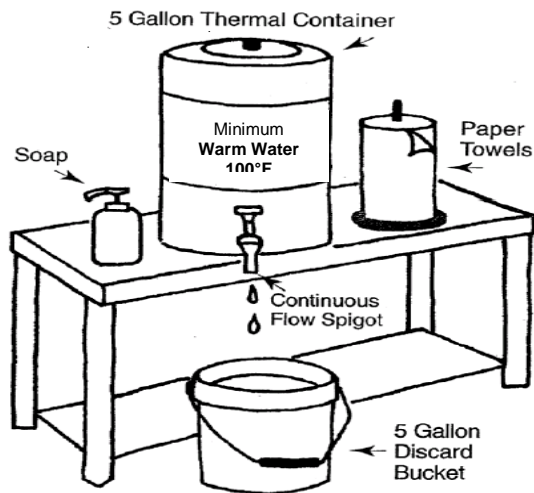
Minimum handwashing sink
